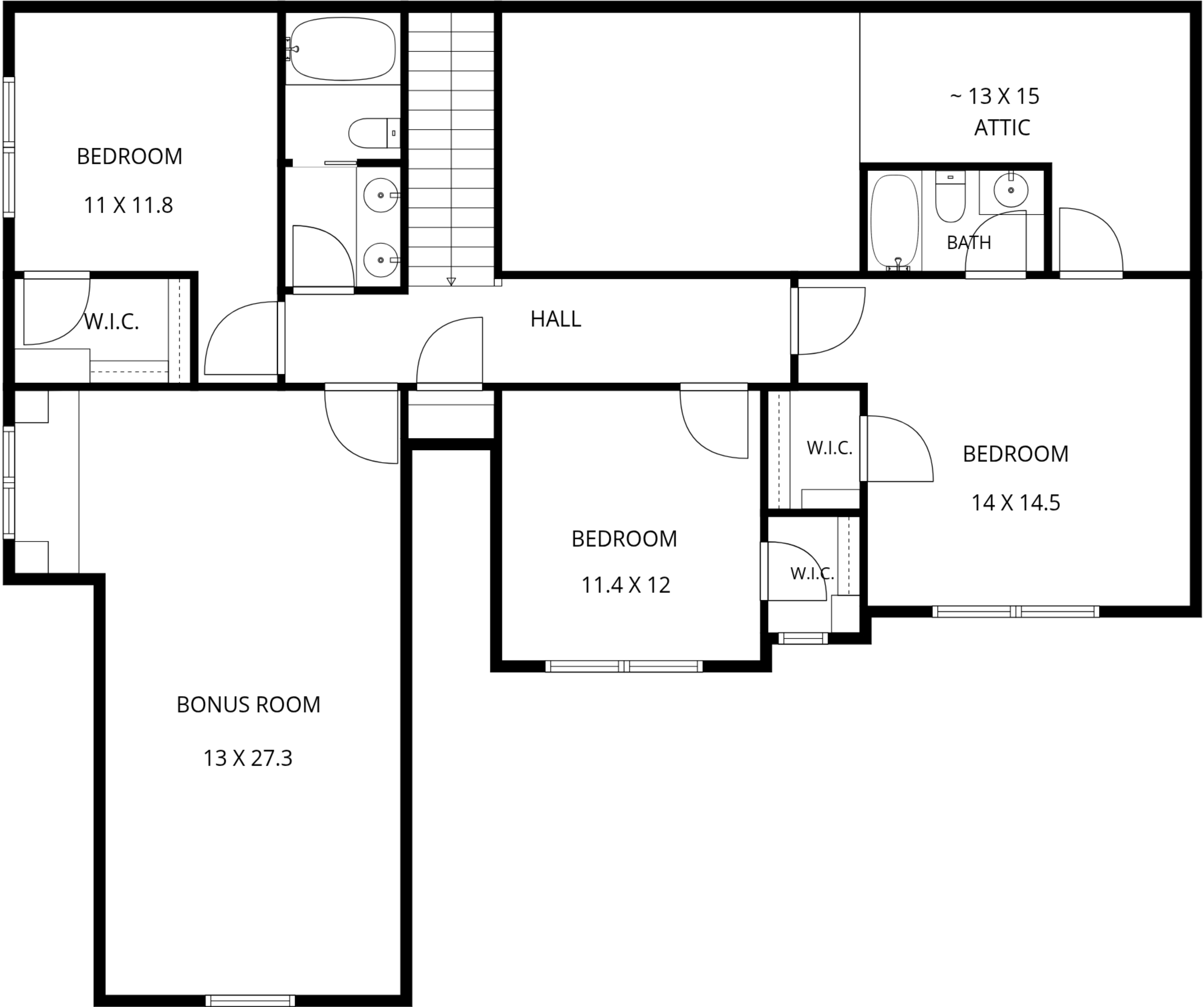
2ND FLOOR
