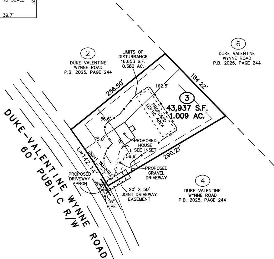
HOUSE 1,084 S.F. PATIO 100 S.F. DRIVEWAY 1,220 S.F. SIDEWALKS 60 S.F. MISC./UTILITIES 18 S.F. TOTAL IMPERVIOUS AREA 2,482 S.F. TOTAL LOT AREA 43,937 S.F. PERCENTAGE OF IMPERVIOUS AREA 5.65 %
