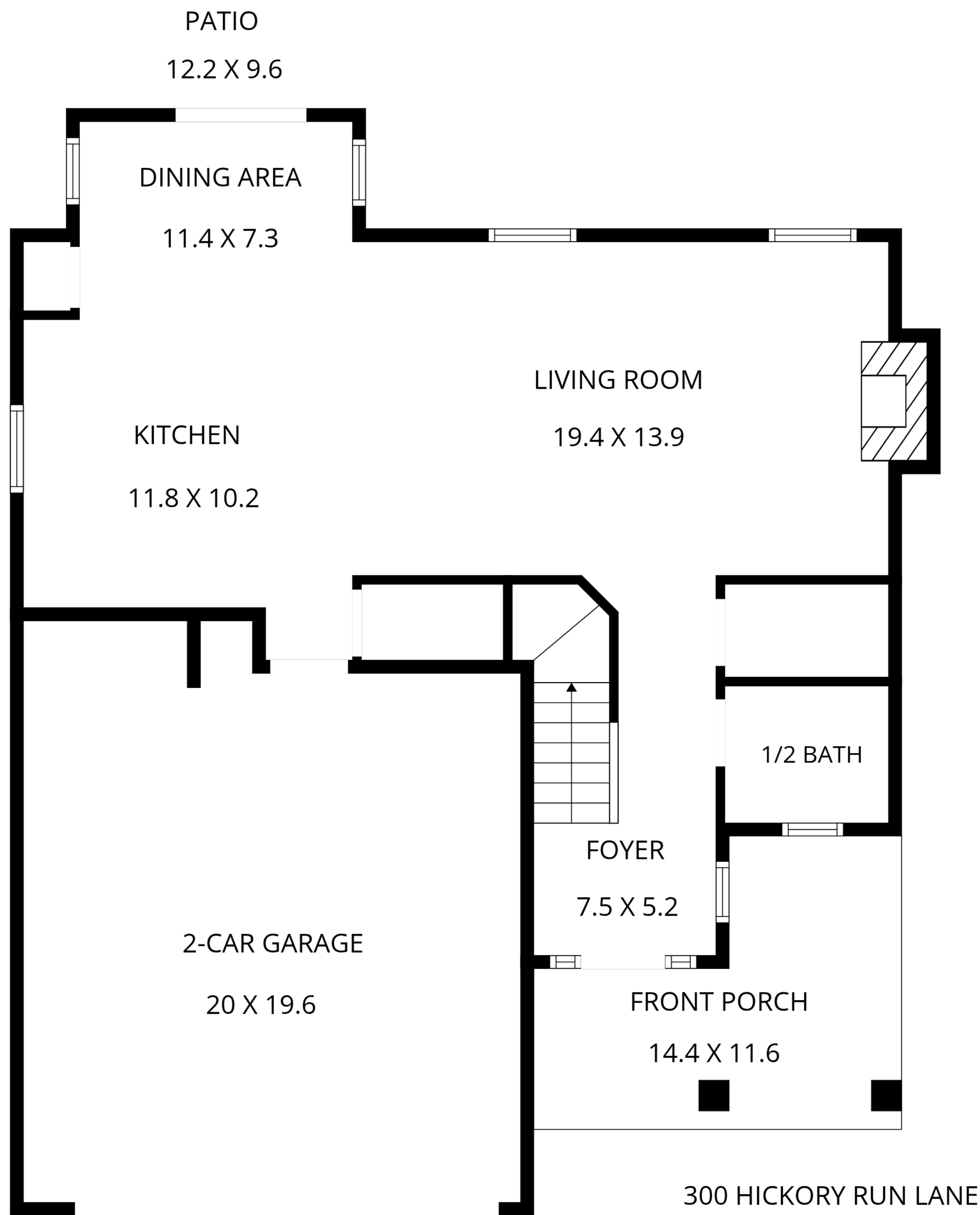
1st floor
