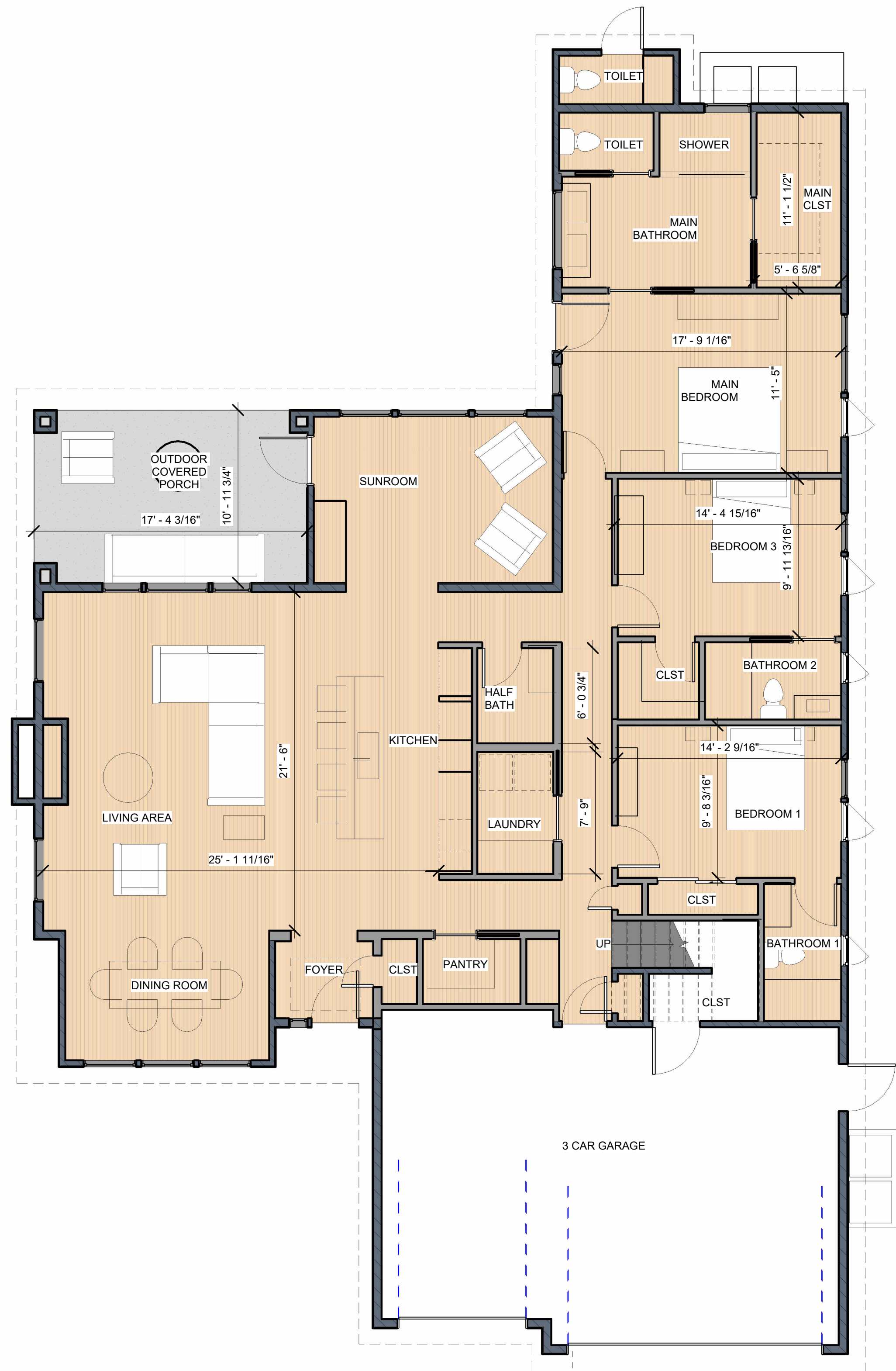
① FIRST FLOOR M 3/16" = 1'-0"
