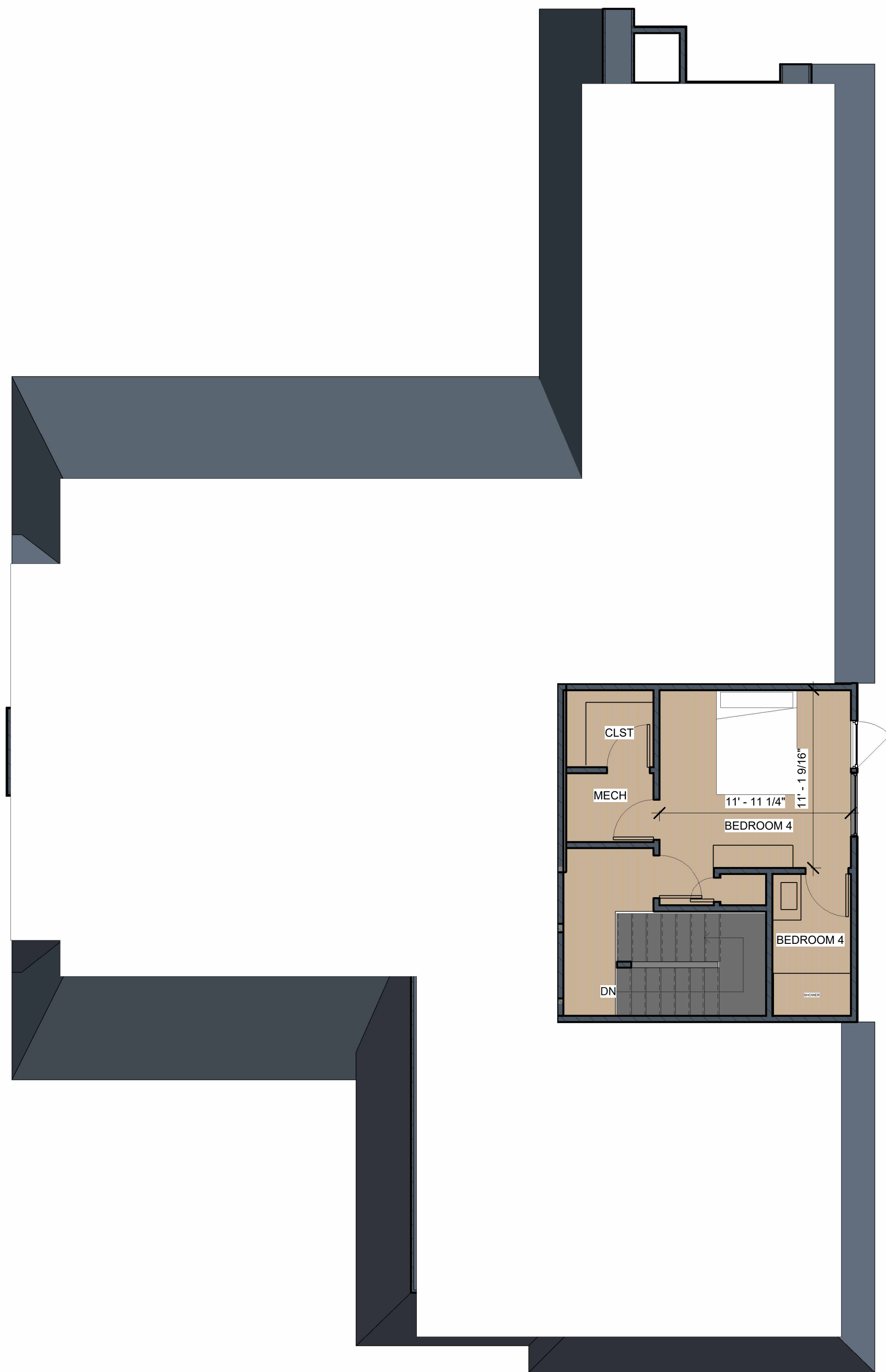
② SECOND FLOOR M 3/16" = 1'-0"
