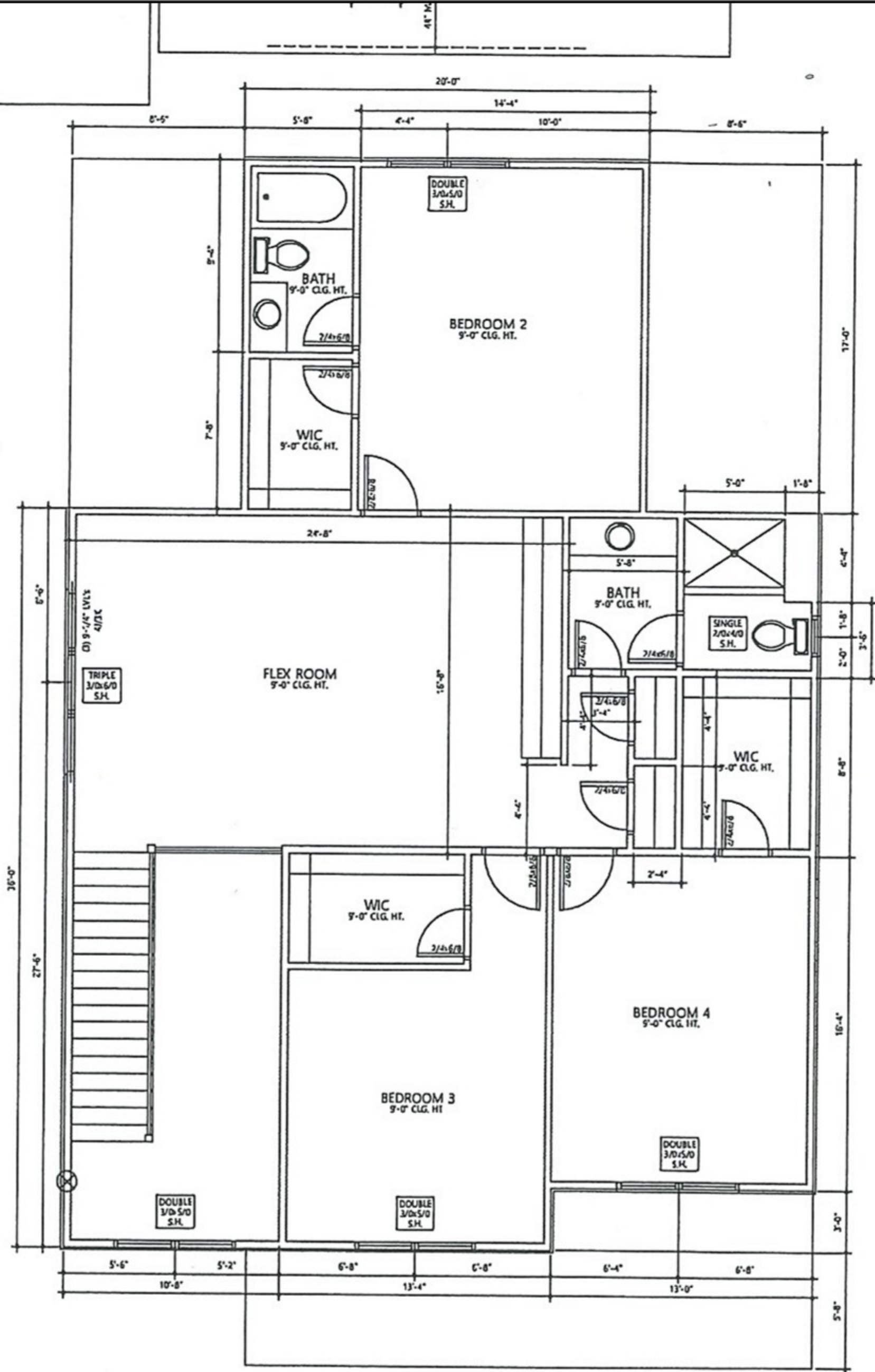
102 UPPER LEVEL PLAN 1/4" = 1'-0" Bl.0
