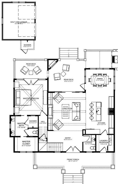
FIRST FLOOR PLAN 1,343 HEATED SQUARE FEET
