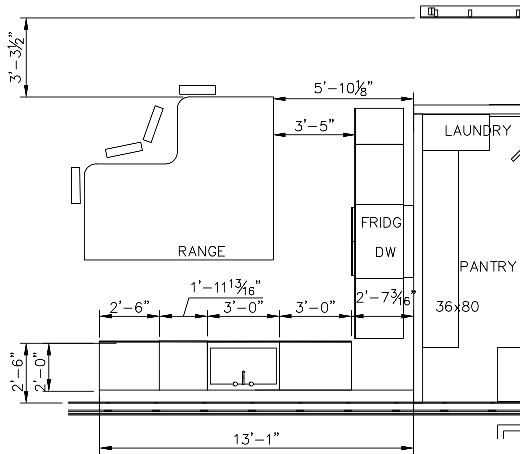
KITCHEN FLOOR PLAN
