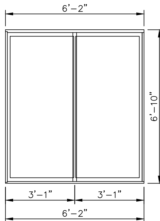
96x80 3 FIXED WINDOW (PD2) (6)
