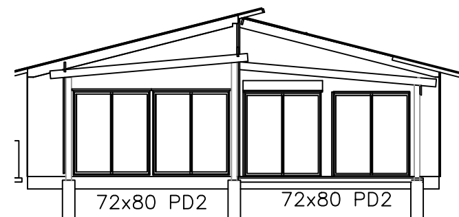
FRONT VIEW SCALE: 3/32" = 1'-0"
