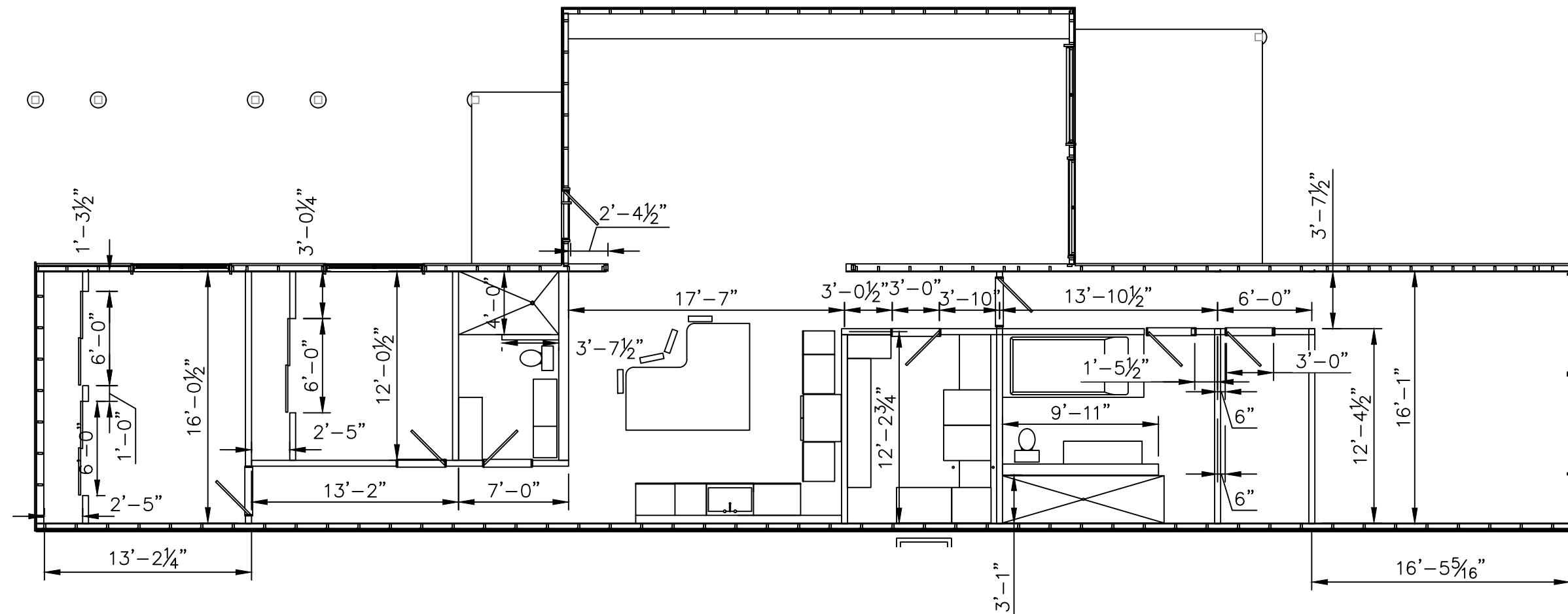
FLOOR PLAN SCALE: 3/16" = 1'-0"
