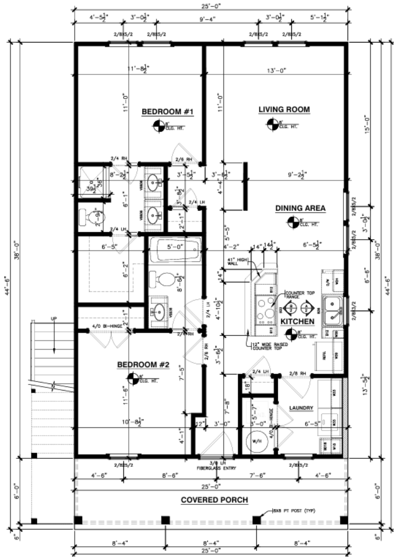
1 2 FIRST FLOOR UNIT "A" PLAN SCALE: 1/4"=1'-0"
