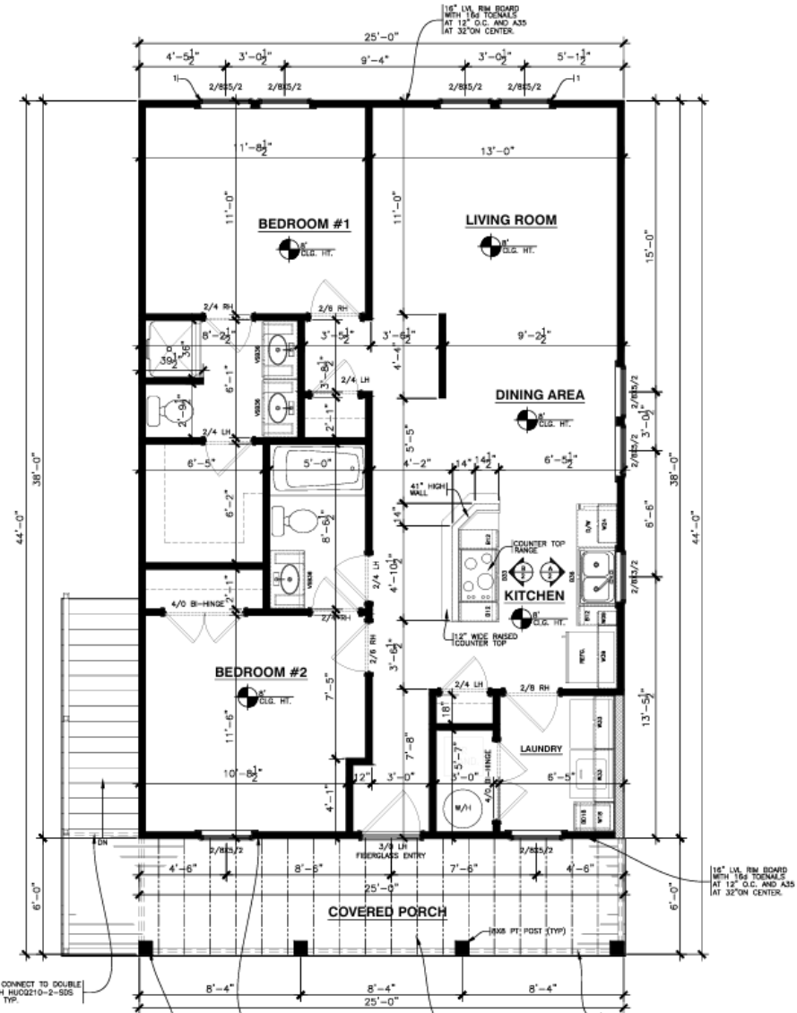
2 2 SECOND FLOOR UNIT "B" PLAN SCALE: 1/4"=1'-0"
