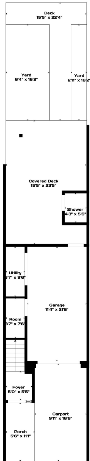
Floor 1
