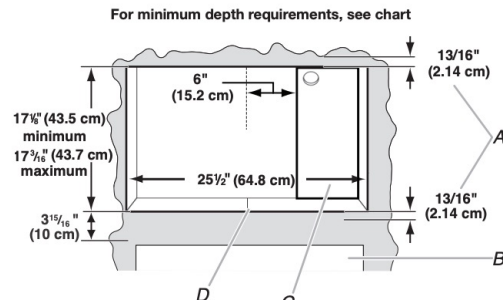
Microwave cutout
