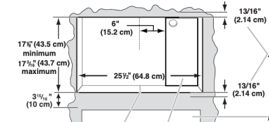
MICROWAVE TRIM KIT
