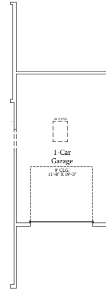
Optional 1-Car Carriage Garage Not Available w/ Opt. 2-Car Side Load Garage or 3-Car Side Load Garage SCALE: 1/4"=1'-0" ON 22x34 AND 1/8"=1'-0" ON 11x17
