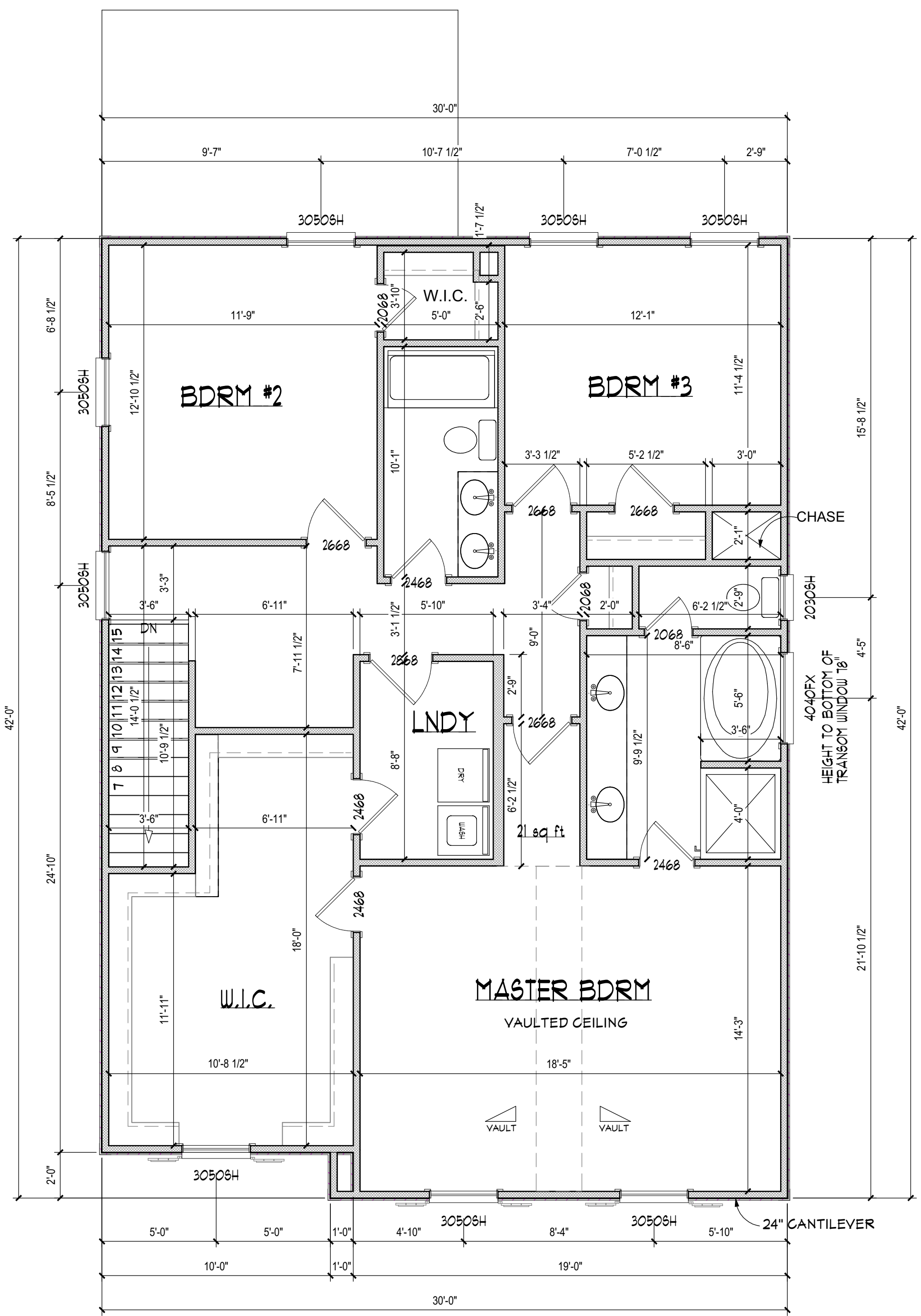
SECOND FLOORPLAN SCALE 1/4" = 1'-0" 1213 sq ft
