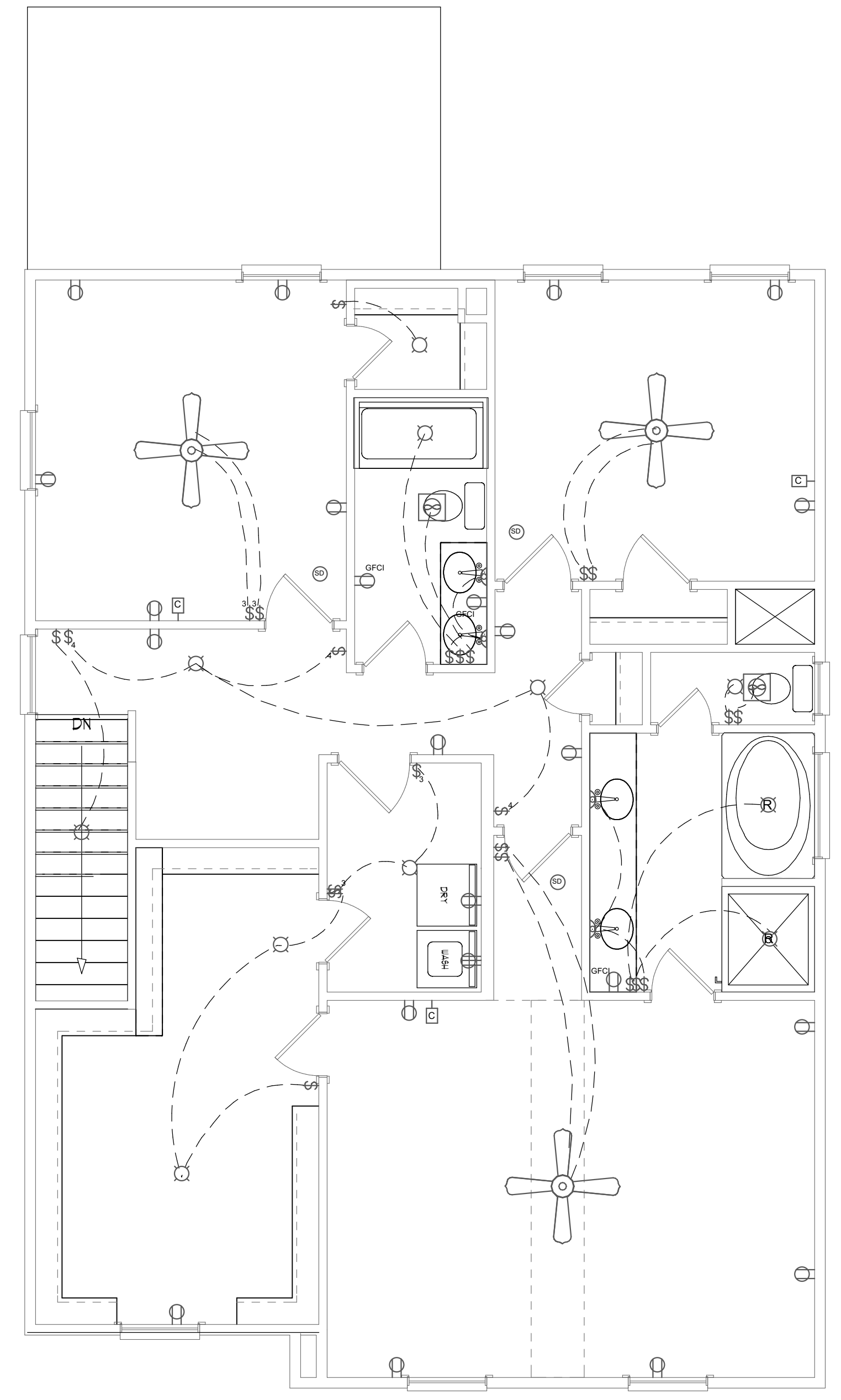
ELECTRICAL PLAN SCALE 1/4" - 1'-0"
