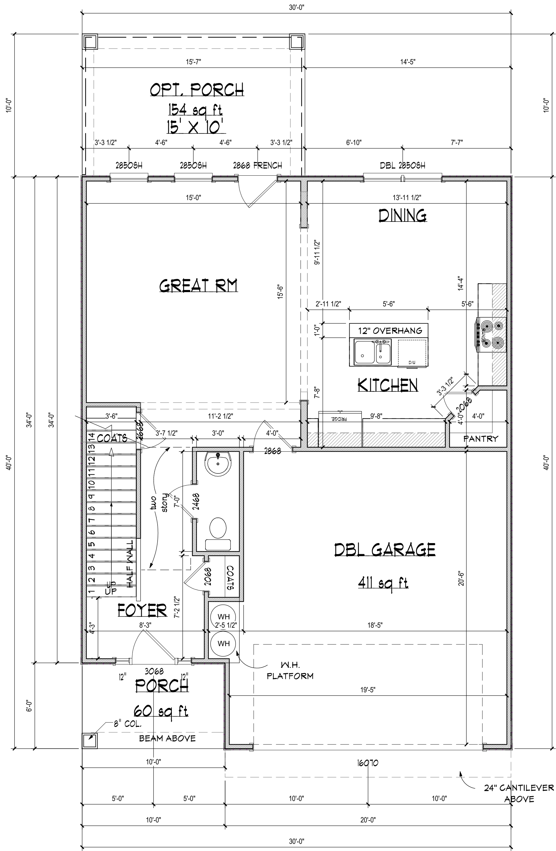
FIRST FLOORPLAN SCALE 1/4" = 1'-0" 742 sq ft
