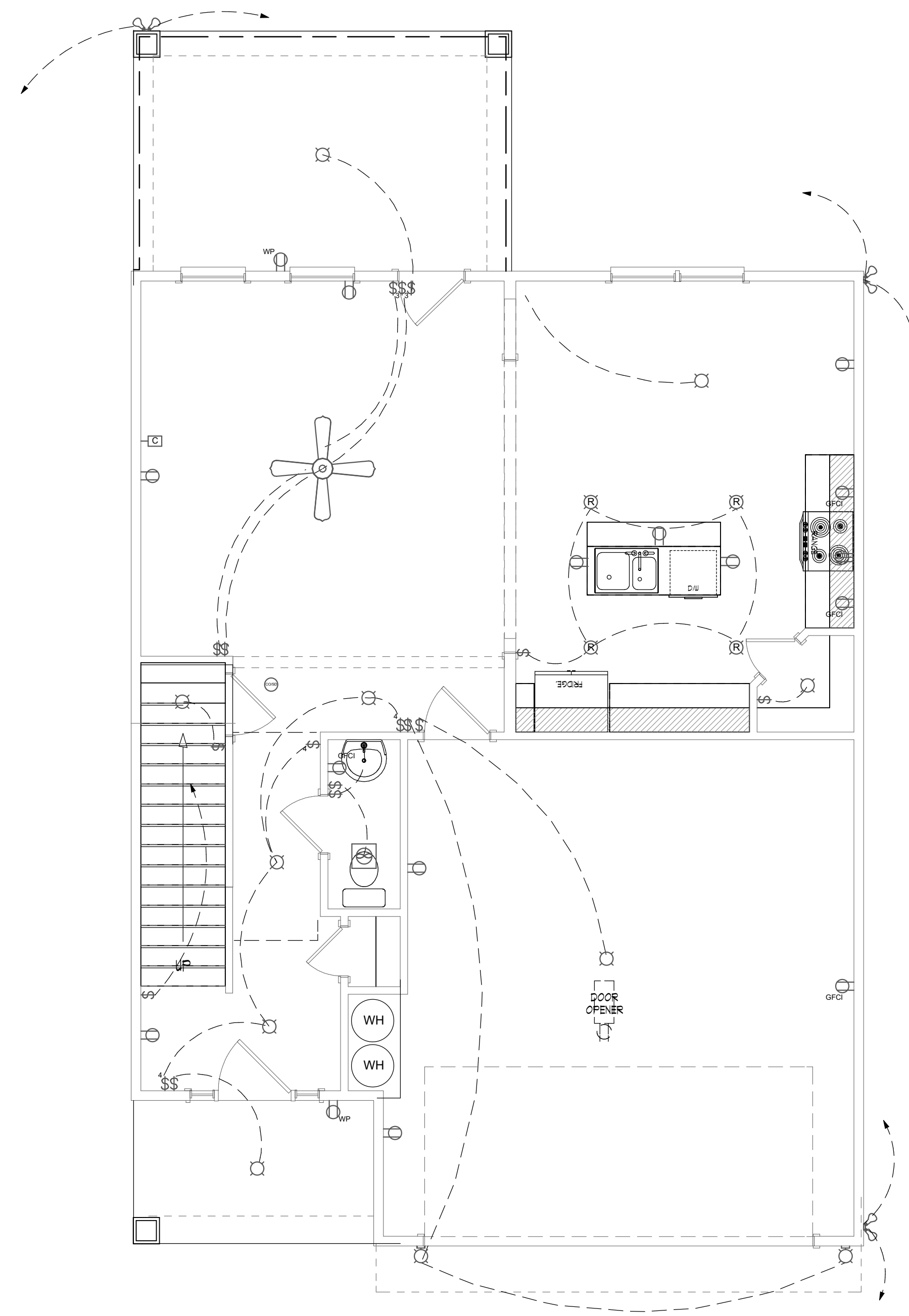
ELECTRICAL PLAN SCALE 1/4" - 1'-0"
