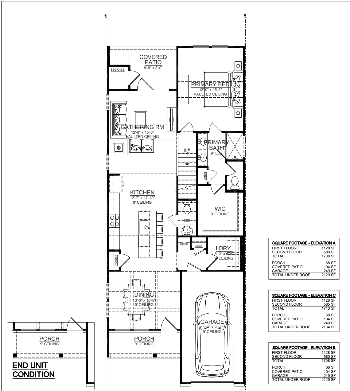
FIRST FLOOR PLAN (ELEVATION A SHOWN)
