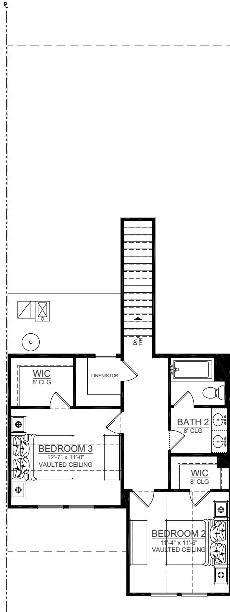
SECOND FLOOR PLAN (ELEVATION A SHOWN)
