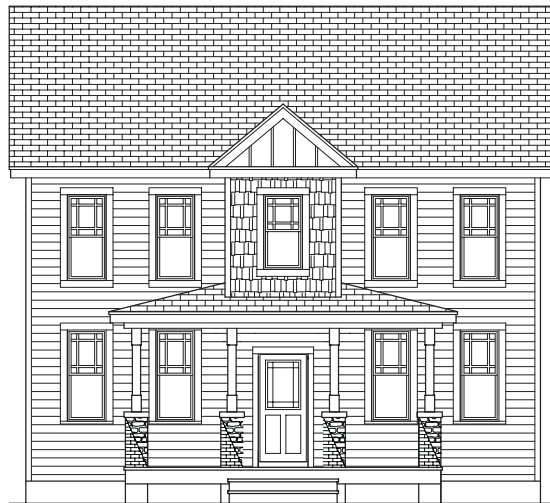
Elevation C
