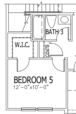
OPT BEDROOM 5/ BATH 3 ILO STUDY (ELEV A SHOWN)
