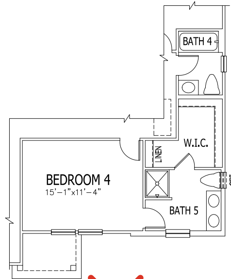
OPT BEDROOM 4/ BATH 5 ILO BEDROOM 3 AND OFFICE
