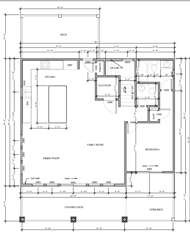
② 2ND FLOOR 1/4" = 1'-0"
