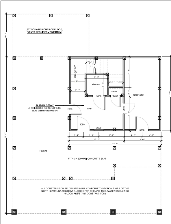
③ GROUND FLOOR 1/4" = 1'-0"
