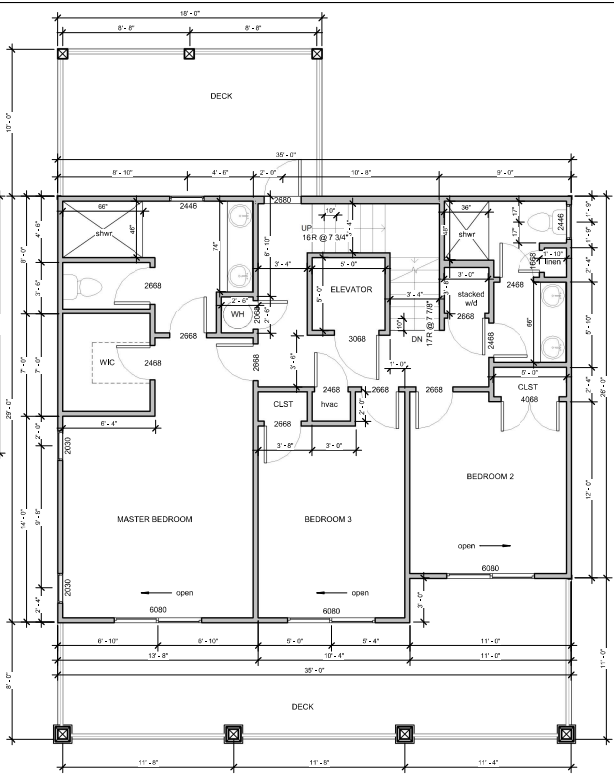
① 1ST FLOOR 1/4" = 1'-0"
