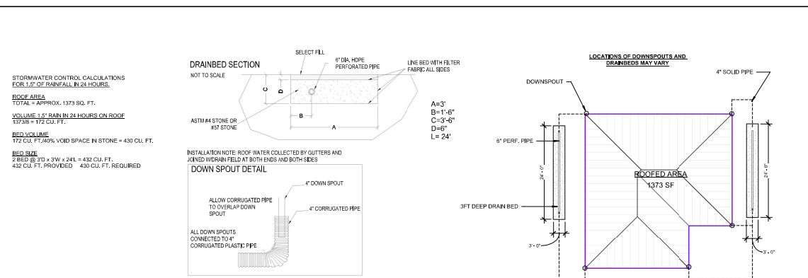
⑤ STORMWATER PLAN 1" = 20'-0"
