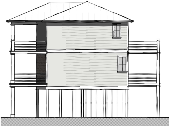
3 RIGHT SIDE 3/16" = 1'-0"
