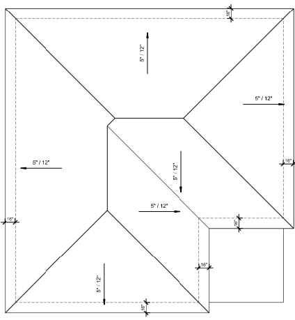
④ ROOF PLAN 3/16" = 1'-0"
