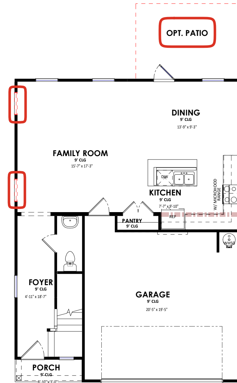
1st Floor Plan - A CS
