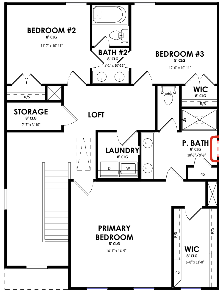
2nd Floor Plan - A CS
