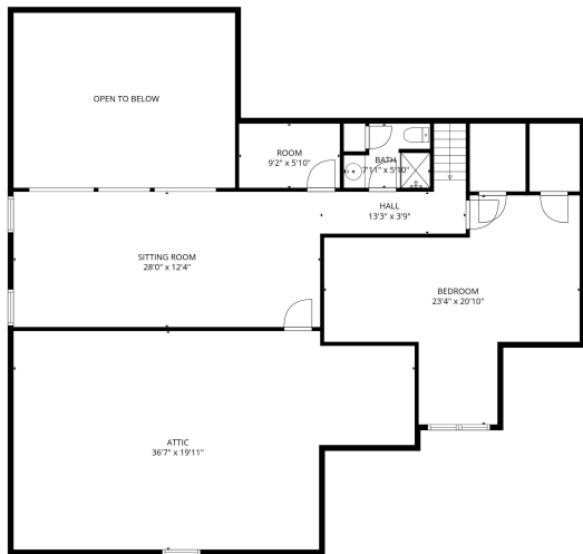
2nd floor
