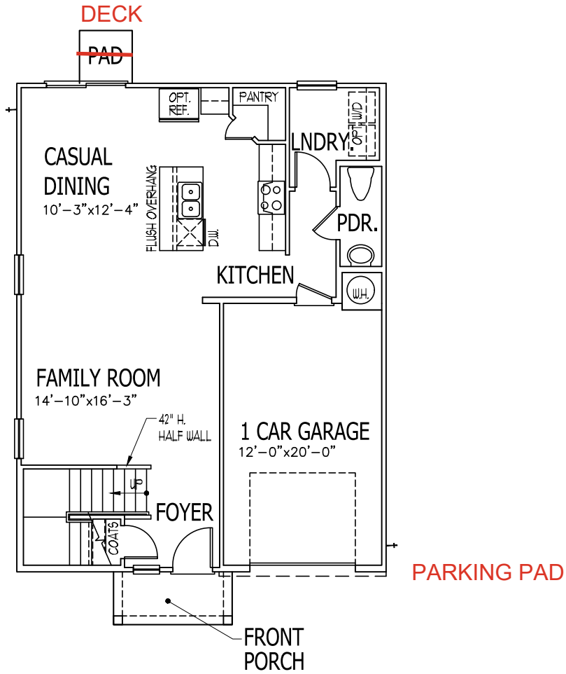
FIRST FLOOR PLAN A AND B
