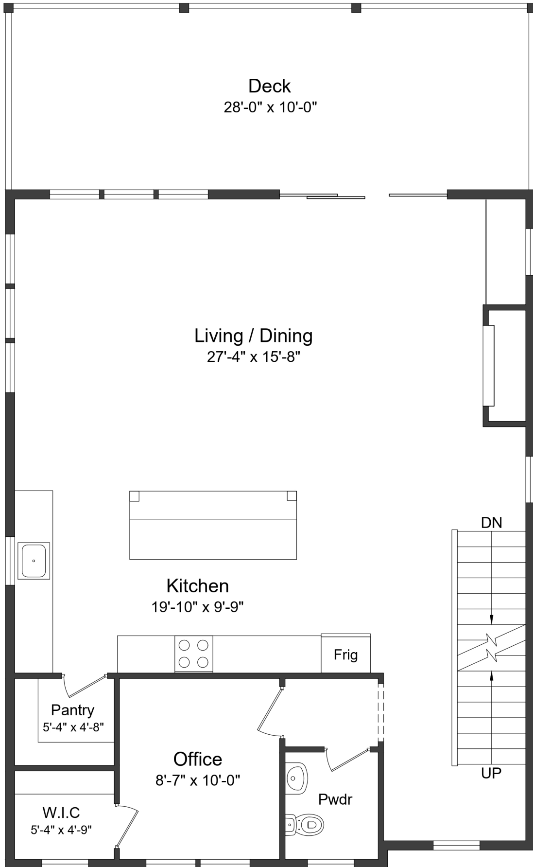
Second Floor
