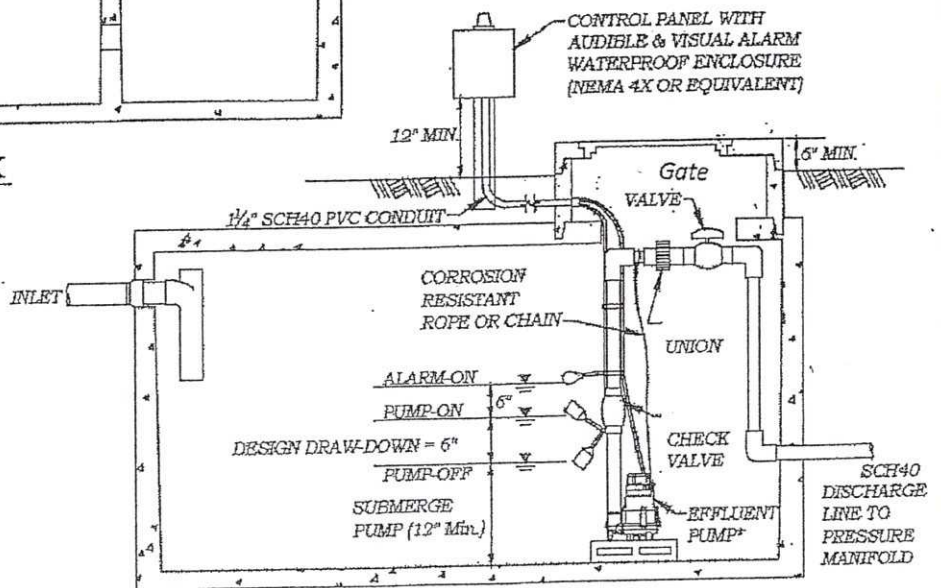
PUMP TANK
