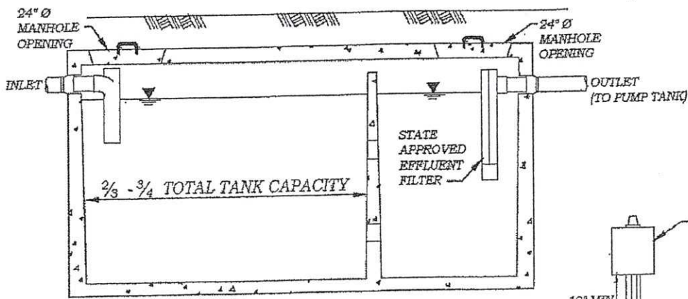
SEPTIC TANK
