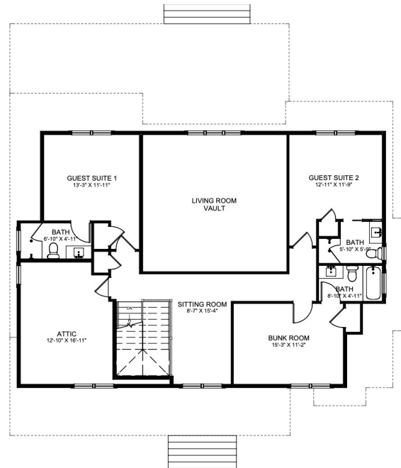
SECOND FLOOR PLAN 1,024 HEATED SQUARE FEET
