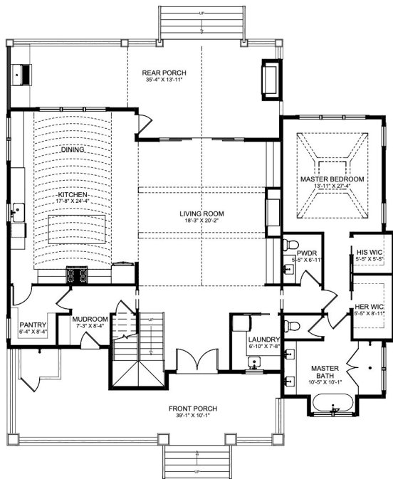
FIRST FLOOR PLAN 1,946 HEATED SQUARE FEET
