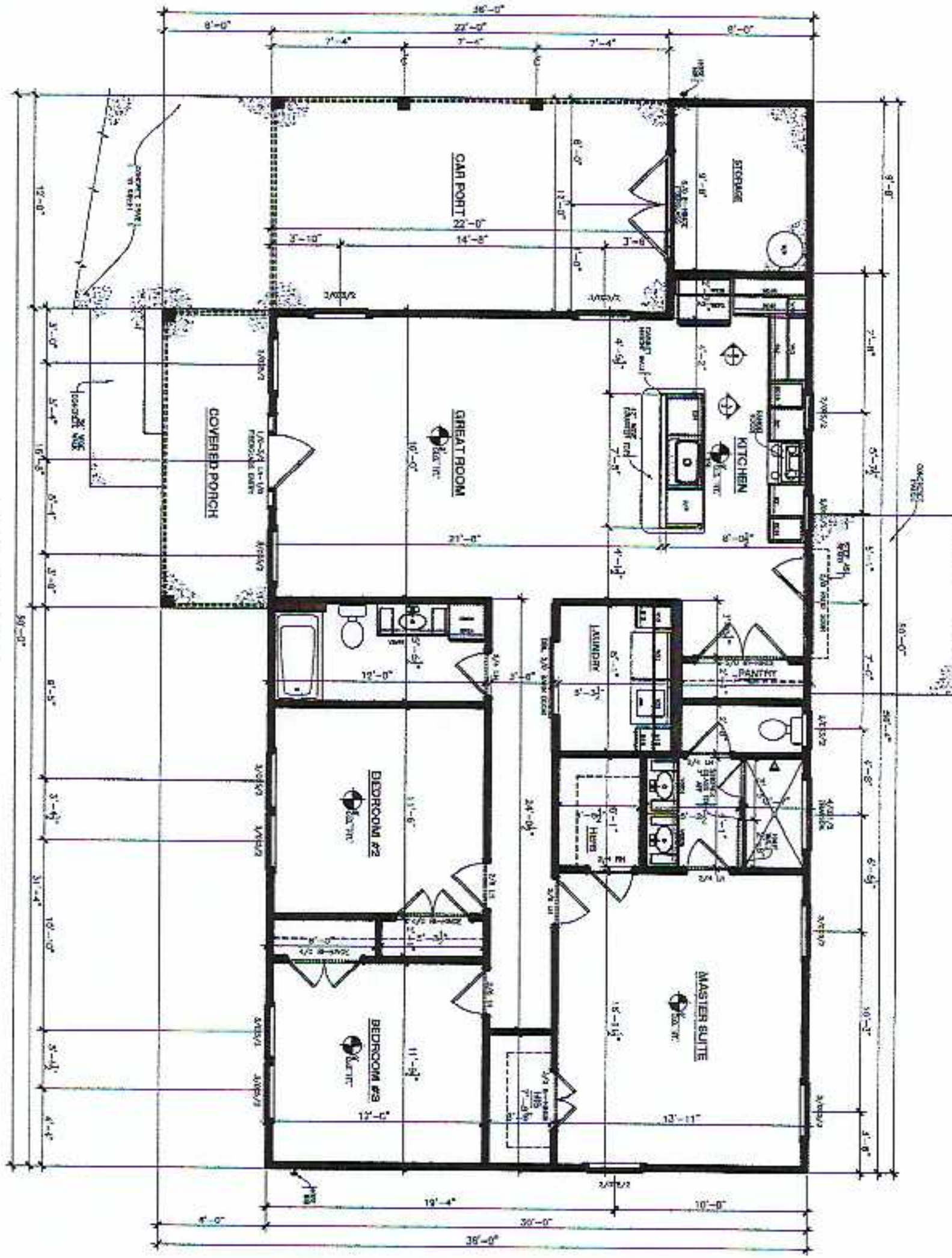
1 FLOOR PLAN
