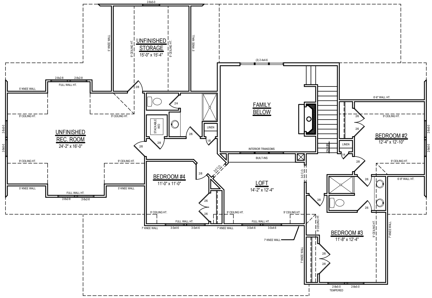
SECOND FLOOR PLAN 1/4" = 1'-0" CEILING HT. = 9'-0"
