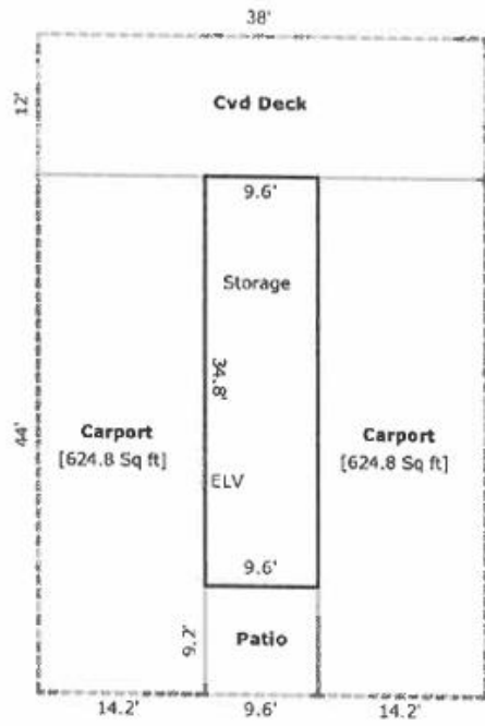
First Floor [334.08 Sq ft]
