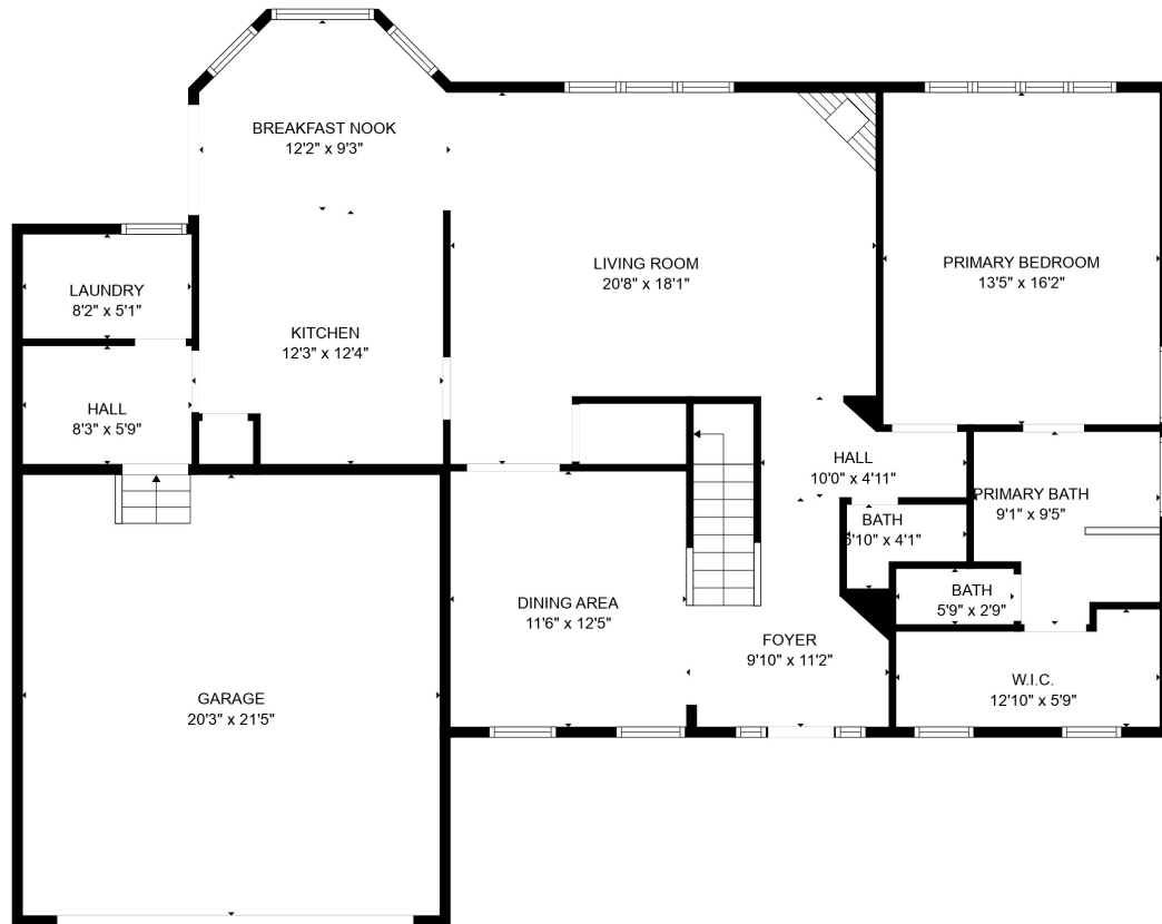
FLOOR 1
